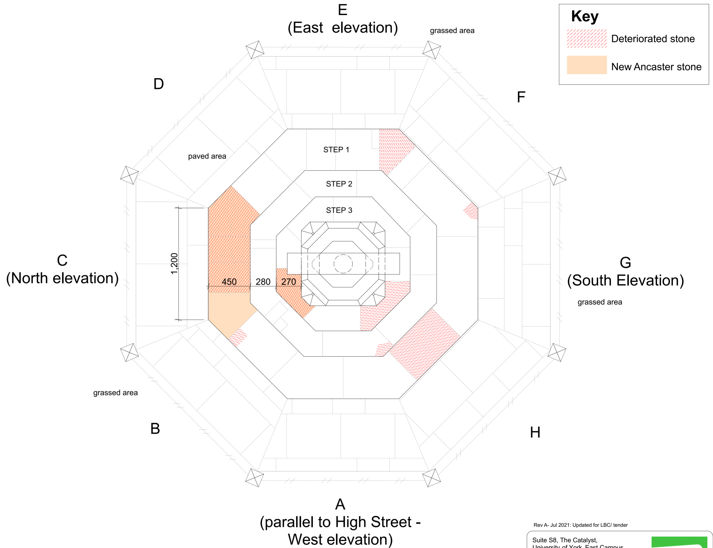
PLAN_EXISTING SCALE 1:20
