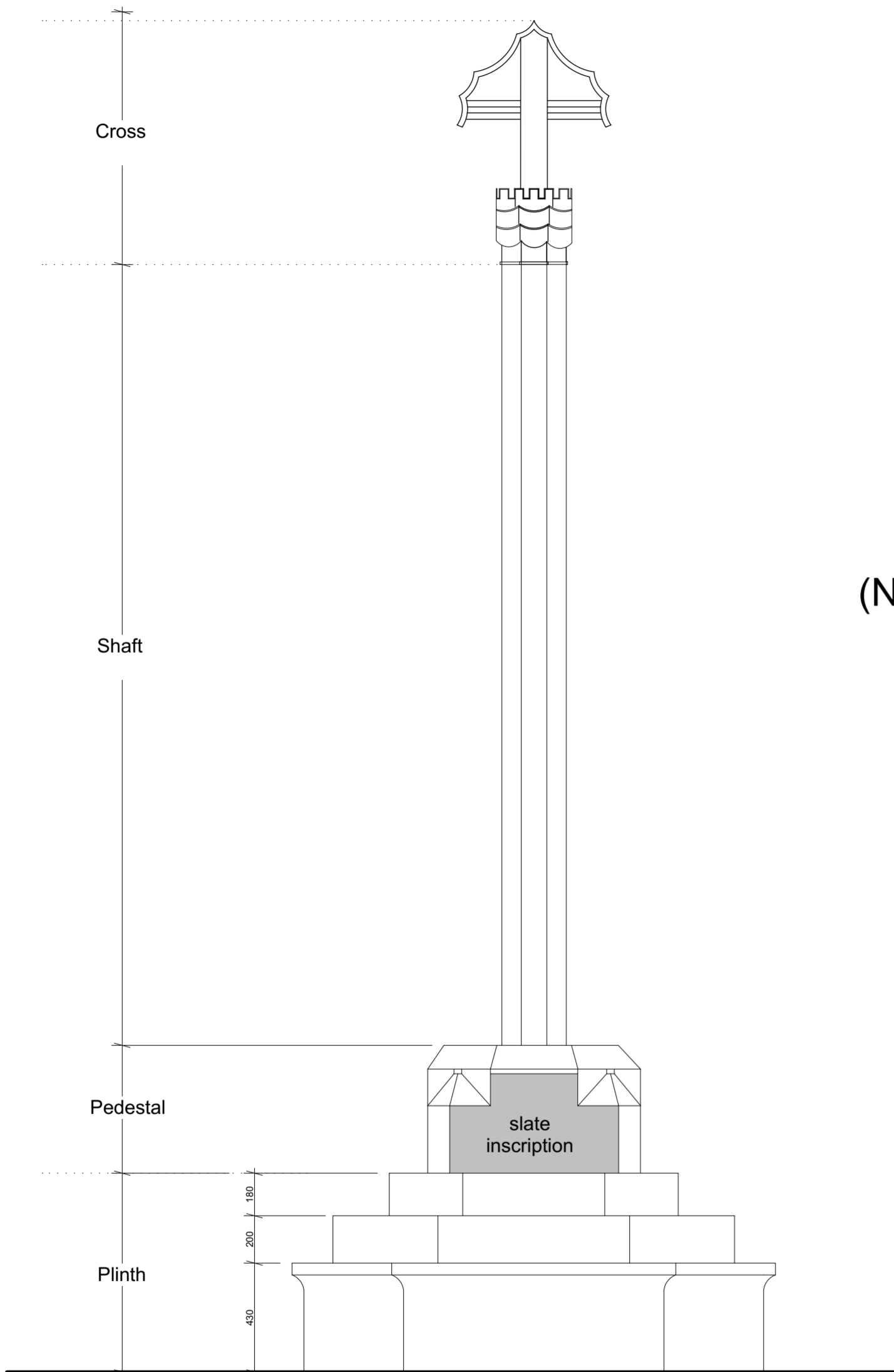
ELEVATION_EXISTING SCALE 1:20
